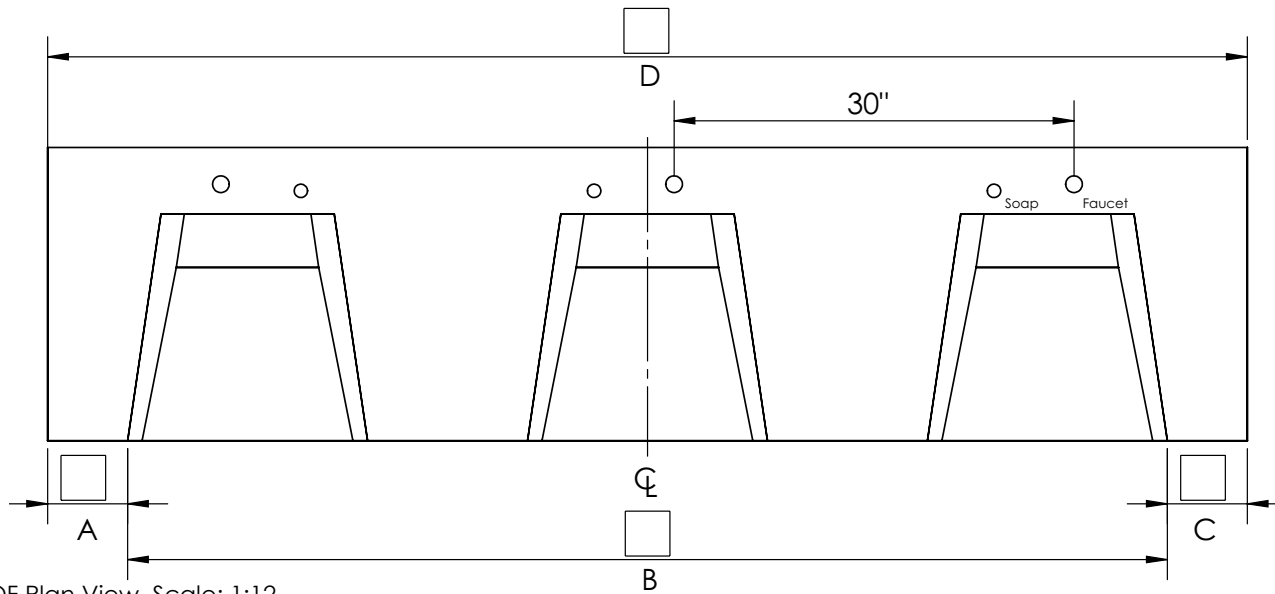
DSOF Plan View Scale: 1:12 Mounting Options
